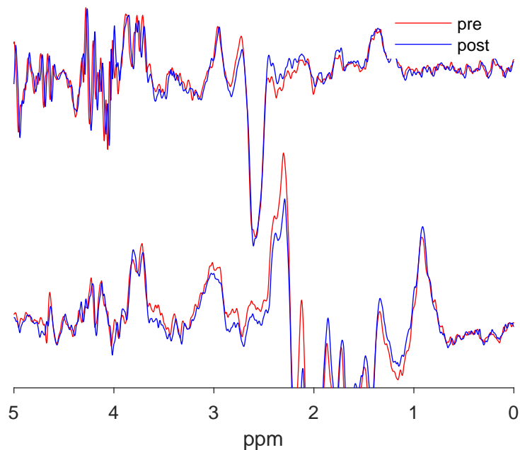
Edited Spectra (pre- and post-alignment)
