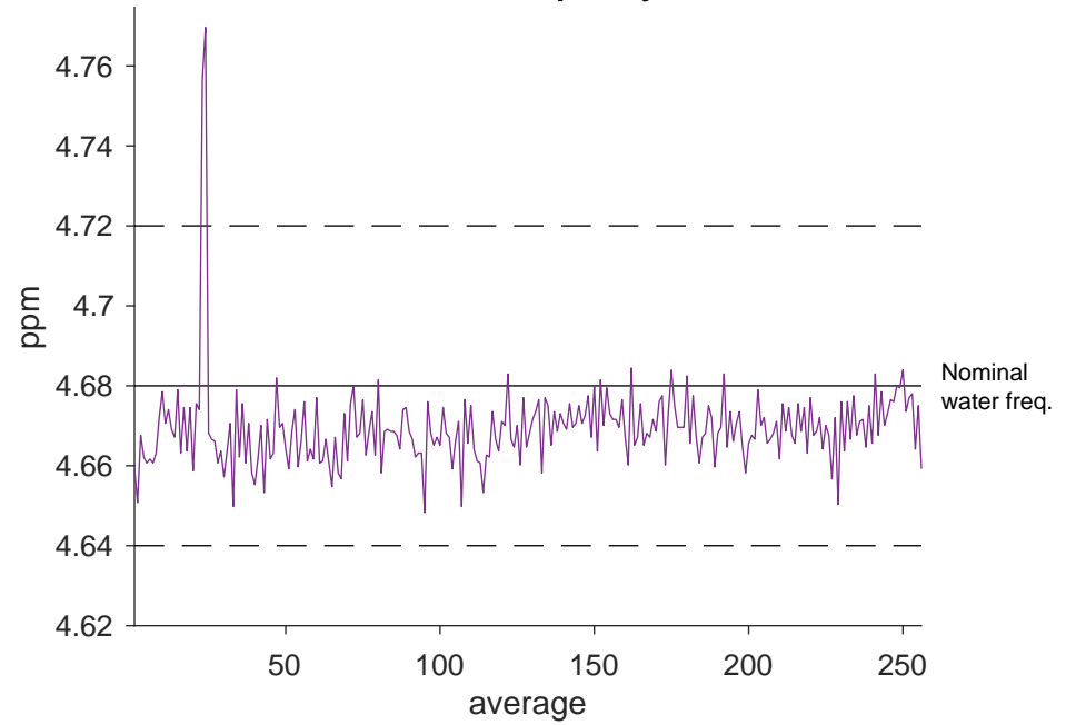
Water Frequency
